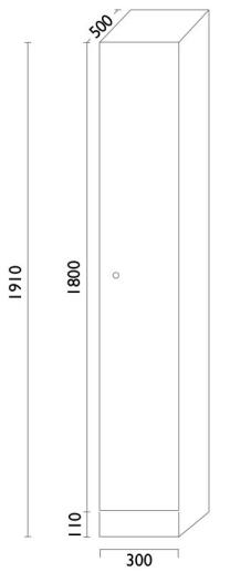
1 Tier Spacious Storage with Hanging Rails
