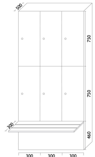
2 Tier Locker Unit with Seating, Hanging Rail and Shelf. Optional: Shoe Box Underneath
