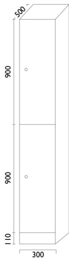
2 Tier Hanging Rail and Shelf
