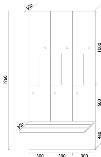
Z Shaped 2 Tier Locker Unit with Seating, Hanging Rail and Shelf
